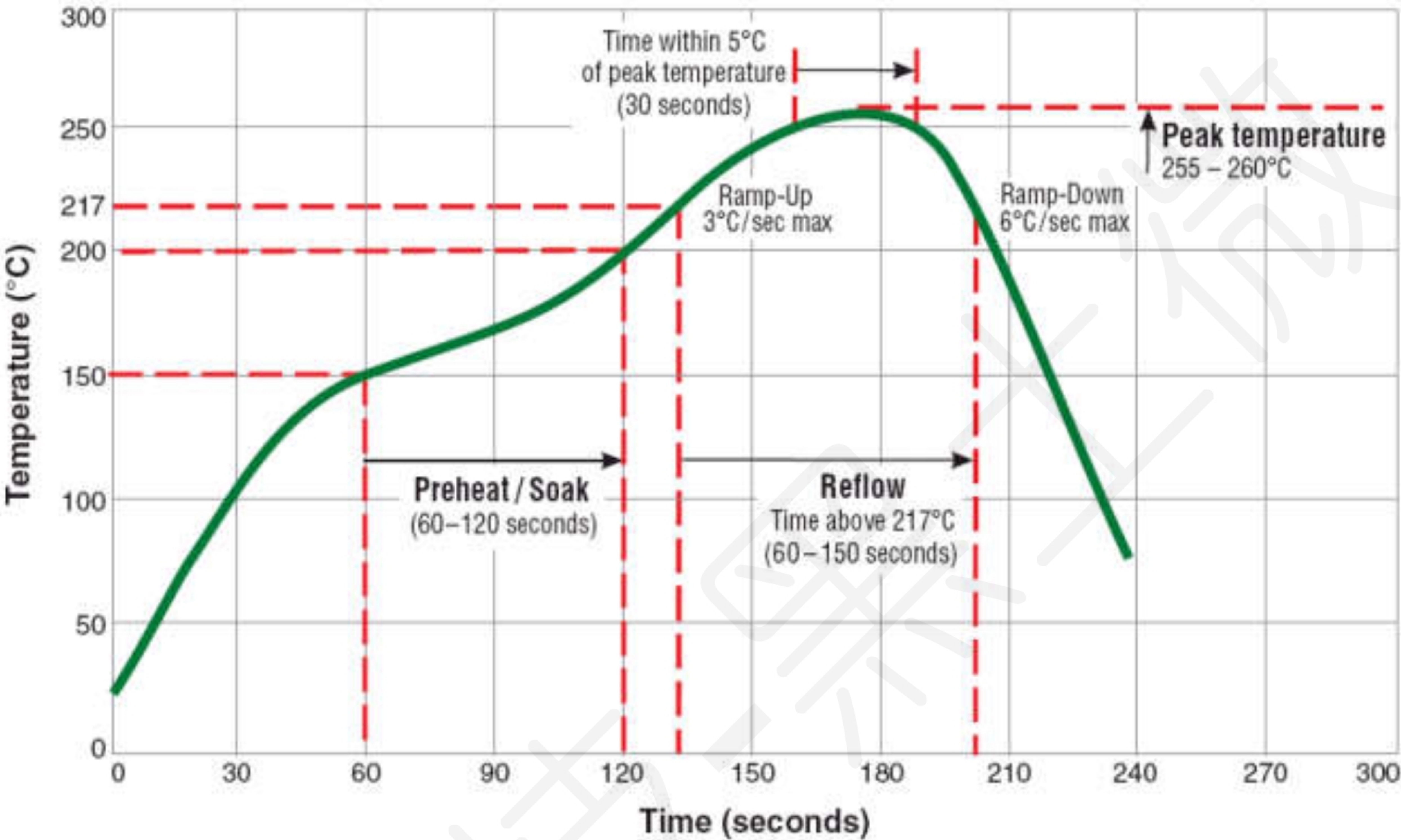
Typical RoHS Reflow Profile
