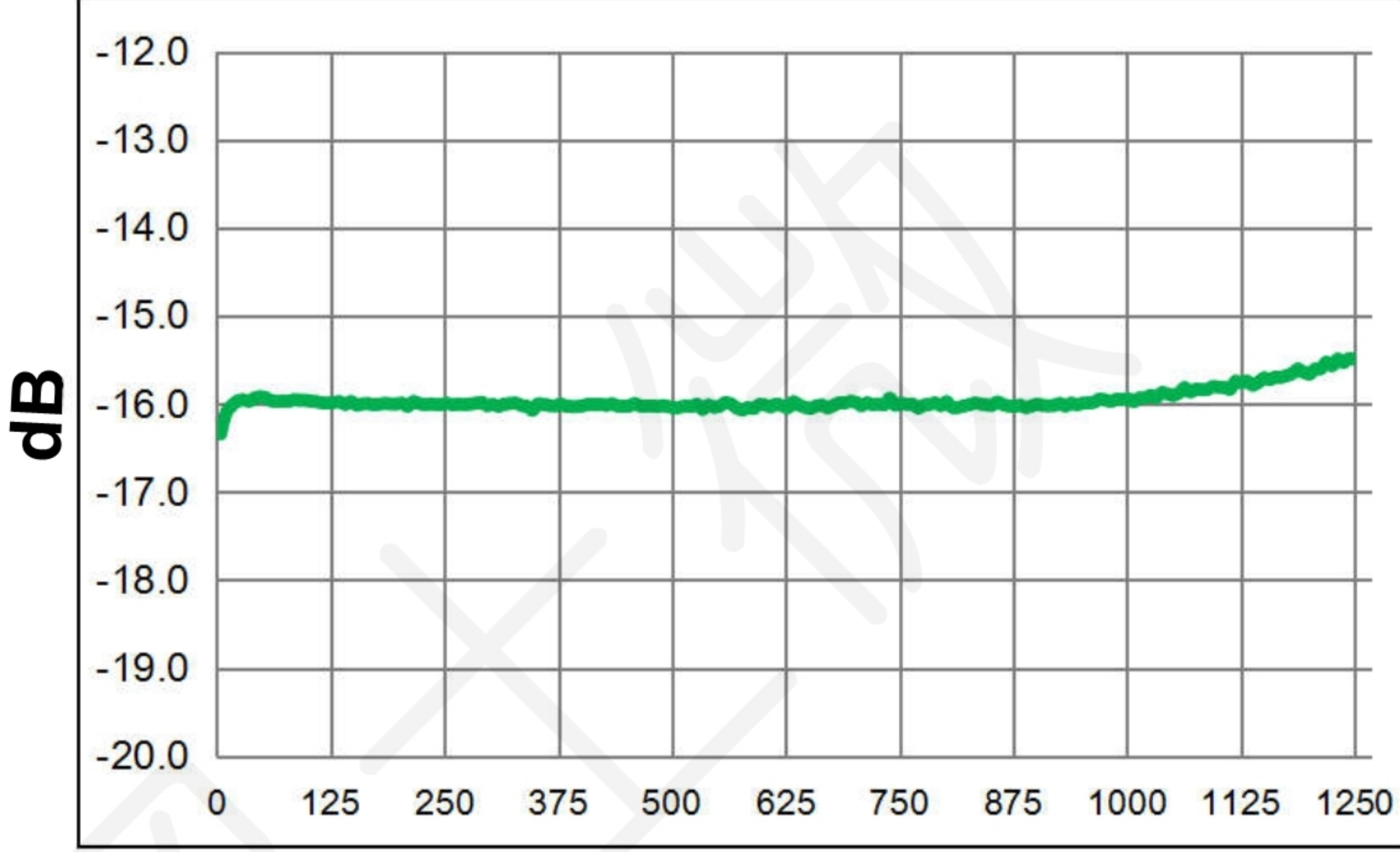
Frequency(MHz)
